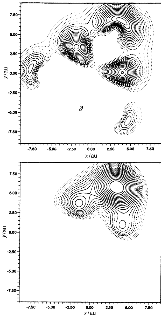
Fig. 10 Sections of the electrostatic potentials for the hypothetical [\text{HMo}_6\text{O}_{19}]^{7-} , away from the triangular anion face containing three terminal and three bridging O atoms at z = 1.1 Å (top) and 2.2 Å (bottom) respectively. Lowest contour: -0.160 hartree (top), -0.11 hartree (bottom). All contour intervals equal to 0.003 hartree (top)- 0.001 hartree (bottom)
