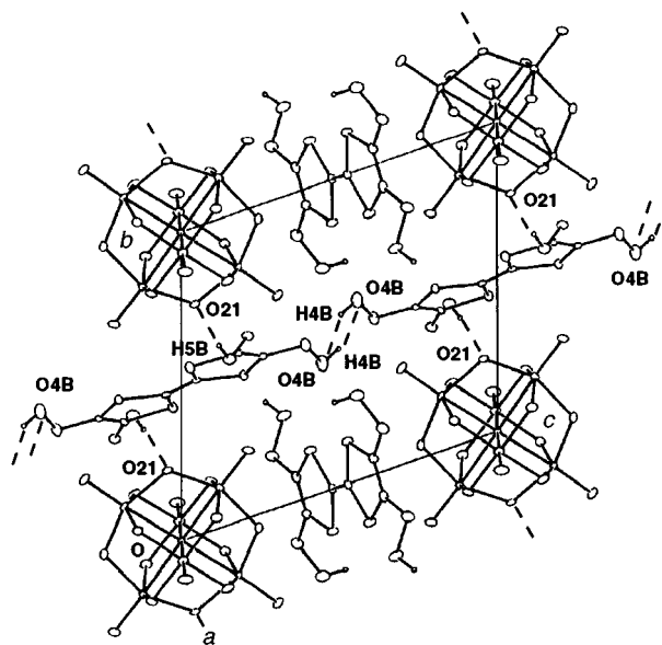
Fig. 5 A projection of the structure of [TTF(CH 2 OH) 4 ] 2 [Mo 6 O 19 ] along the a axis. Both [Mo 6 O 19 ] 2- and TTF(CH 2 OH) 4 2+ moieties are located on inversion centers, at the corners of the cell and the center of the edges respectively. Note the hydrogen bond H4B...O4B cyclic motif as well as the H5B...O21 donor-polyanion hydrogen bond.
