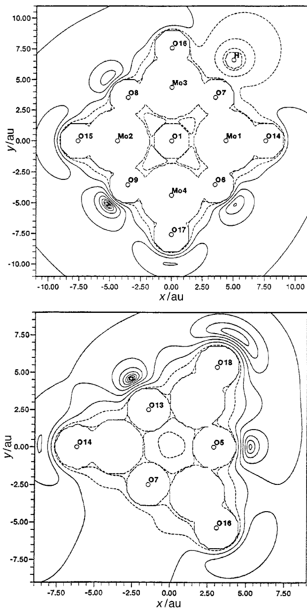
Fig. 9 Sections of the electrostatic potentials for the hypothetical [\text{HMo}_6\text{O}_{19}]^{7-} , in the plane containing four Mo, four terminal and four bridging O atoms (top) and in the plane containing three terminal and three bridging O atoms (bottom); the H atom is linked to O7 which pertains to both planes. Lowest contour: -0.18092 hartree (top), -0.15167 hartree (bottom). First contour interval: 4 \times 10^{-5} hartree. Successive contour intervals increased by a factor of 2.
